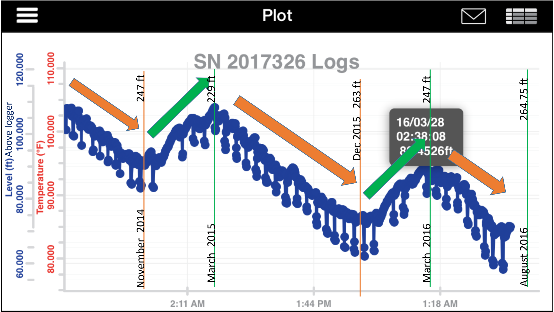
May 2014 to date continuous water level record, Key Well area, Carne and Grand
